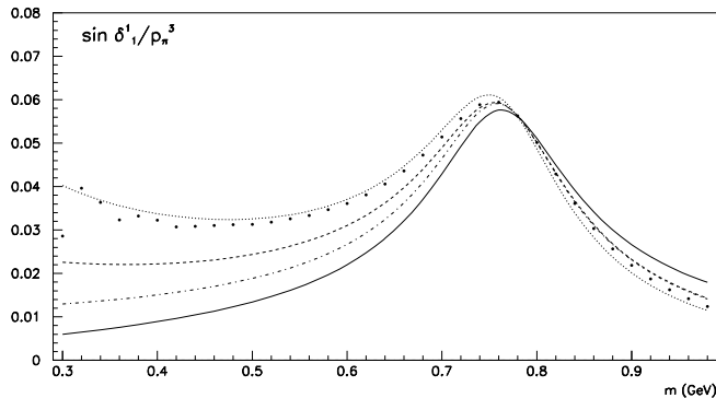
Figure 1: Function \sin \delta_1^1/p_\pi^3 deduced from \pi^+\pi^- phase shifts; the function is given in units of m_\pi^{-3} . The dots correspond to the points of Ref. 8 . Full line is VMD1, dashed line is VMD2, dotted line is HLS (the best description of expected phase) and dashed-dotted is WCCWZ.
